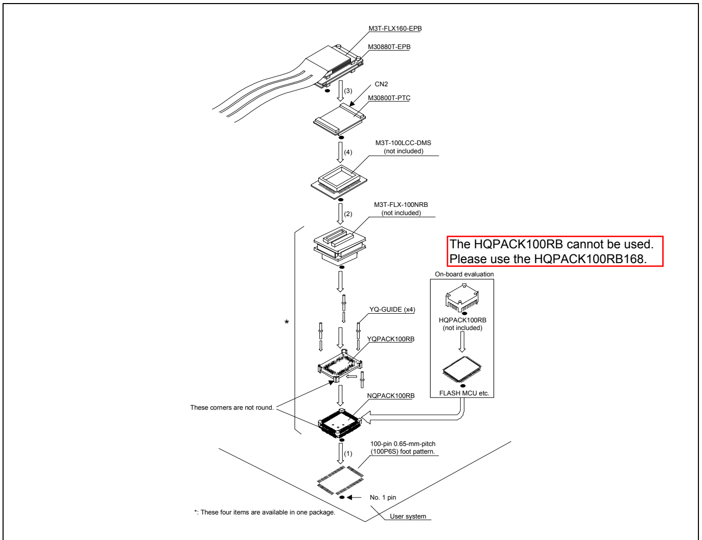
Figure 2.11 Connecting to a 100-pin 0.65-mm-pitch foot pattern (3/3)
